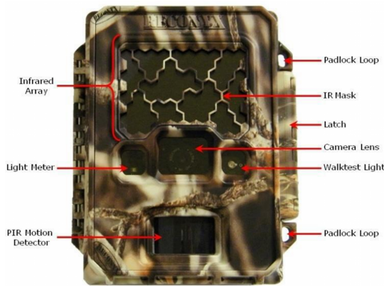
Figure 3 – Diagram of a Reconyx HC600 depicting the main components of a camera trap (Copyright Reconyx Inc.).
